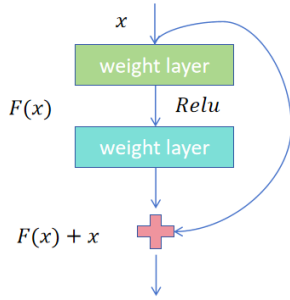
Figure 2: Residual Network Structure
