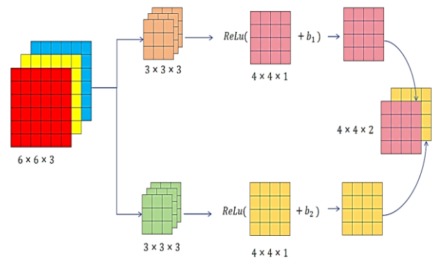
Figure 1: CNN network
