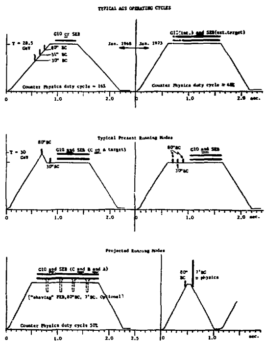
Fig. 2. Typical AGS Operating Cycles.
