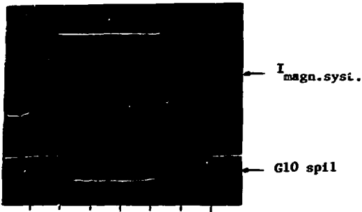
Fig. 1a \rightarrow t (0.5 sec/cm) AGS Internal Target Spill (G10), Duty Cycle 54%
