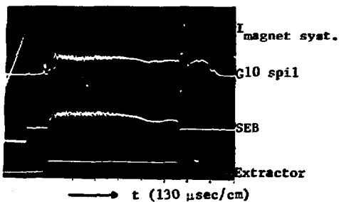
Fig. 1b Simultaneous Operation Internal Target (G10) and Slow External Beam. Duty Cycle \approx 40%.
