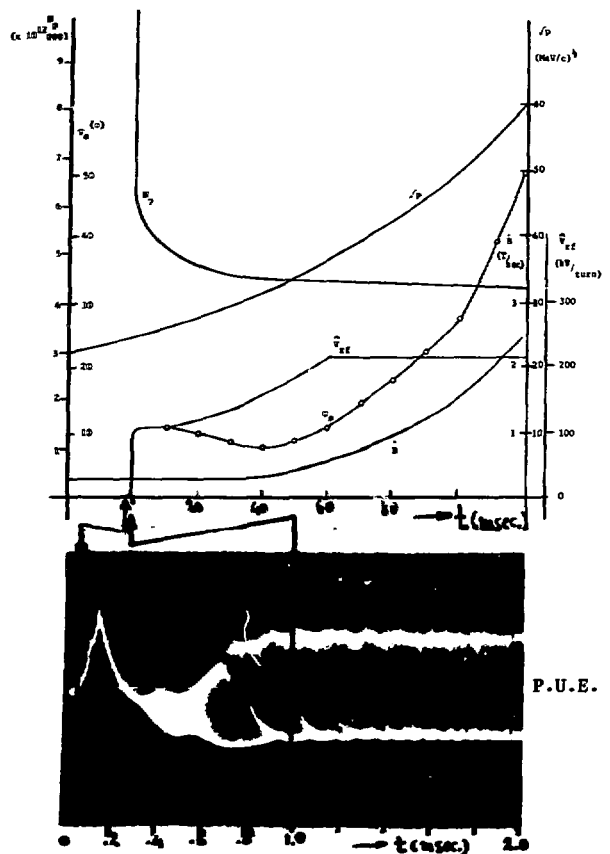
Fig. 3. Injection Parameters and Bunch Formation During "Quasi" Adiabatic Capture.
