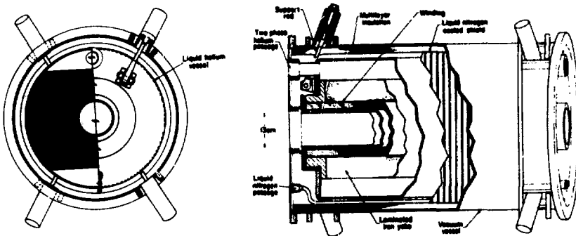
Figure 3 - Dipole magnet with iron inside cryostat (elevation)
