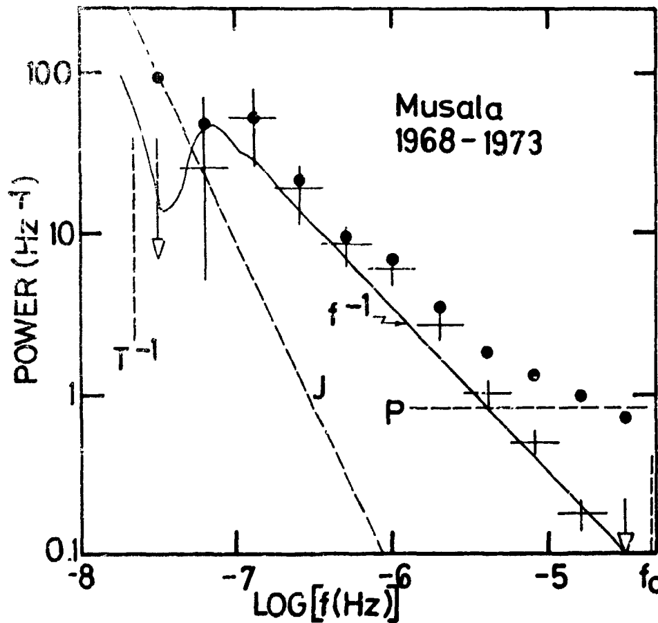
Fig. 1 Power spectra of the Musala fluctuations. Filled circles are the raw spectrum of n_p . Poisson noise level ("p") and contribution of counter-tube jumps ("j") are shown. Heavy bars give "observed spectrum" raw spectrum minus p and j spectra with 1\sigma confidence intervals. Solid curve is predicted result for a f^{-1} spectrum with linear trends subtracted, displaced vertically for clarity. Aliasing frequency is f_c .
