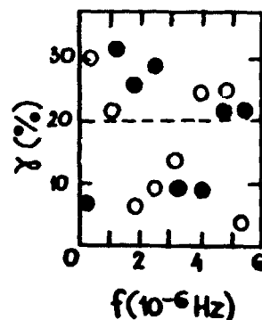
Figure 3 Coherence between Musala and Pressure and Deep River. \gamma(f) is shown for cross-power spectra of Musala and pressure (solid circles) and Musala and Deep River Neutron Monitor (open circles), each with \nu=50 degrees of freedom. Dashed line at \gamma=0.2 gives bias level to be expected from uncorrelated data.
