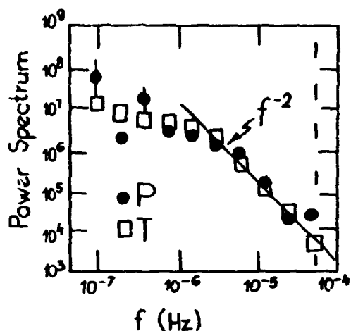
Figure 2 Power spectra of meteorological data. Filled circles and squares give spectra of pressure (in mbar) and temperature (of the P-120 mbar level, in ^{\circ} K). Some 10 confidence intervals are shown; they are smaller for higher frequencies.
