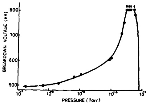
Fig. 7 Hydrogen pressure in the column vs. breakdown voltages. \uparrow denotes that the voltages is not limited by the column.
