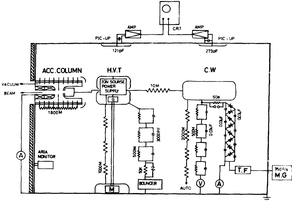
Fig.2 Schematic diagram of high voltage apparatus.
