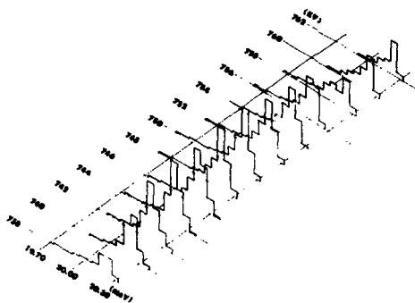
Fig.8 Injection energies vs. energy spread of linac beam.
