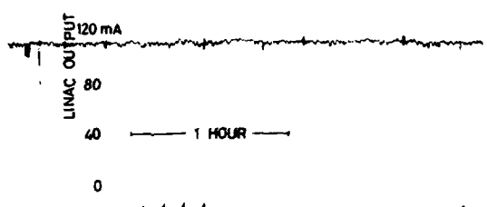
Fig.5 Continuous current variation for linac output.
