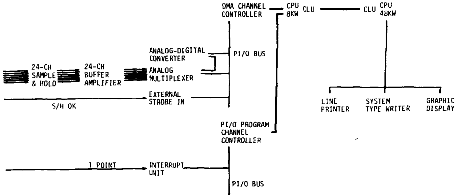
Fig.15 A block-diagram of the computer controlled emittance measurement.
