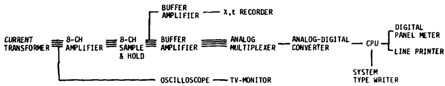
Fig.4 Electronic diagram for digital display.
