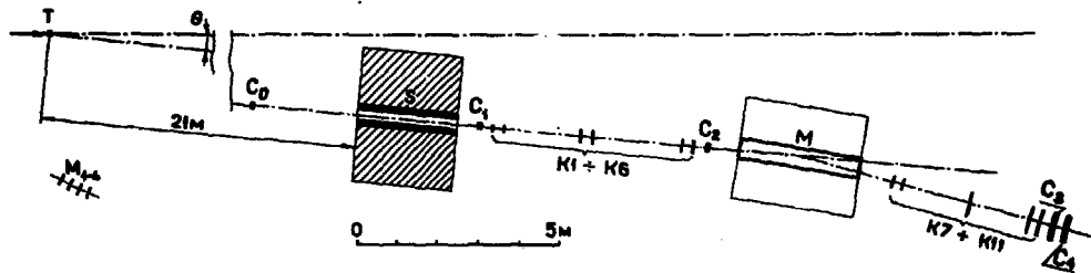
Fig.1. Experimental arrangement. T - target, S - shield, M - analyzing magnet, C_0, \dots, C_4 - scintillation counters, K_1, \dots, K_{11} - double - coordinate wire spark chambers, M_{1-4} - monitor.
