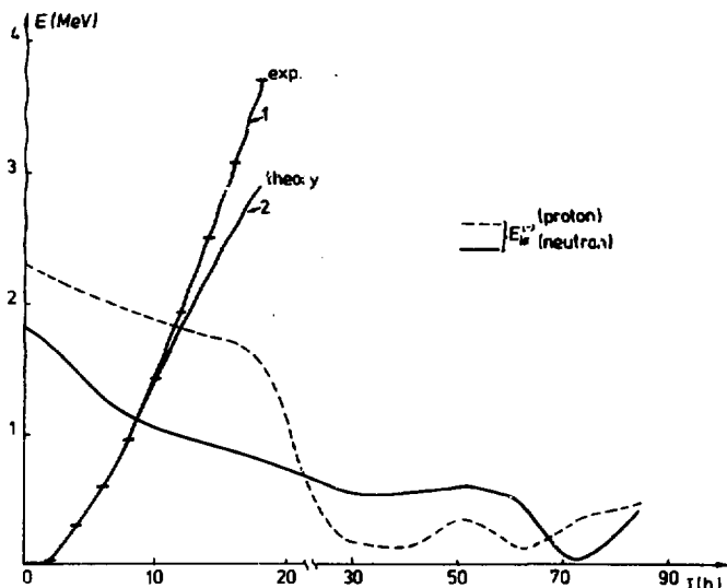
Fig.2. Lowest two-quasiparticle energies E_{ik}^{(-)} as functions of spin and the experimental (1) and calculated (2) energies of the yrast states in ^{168}\text{Yb} .
