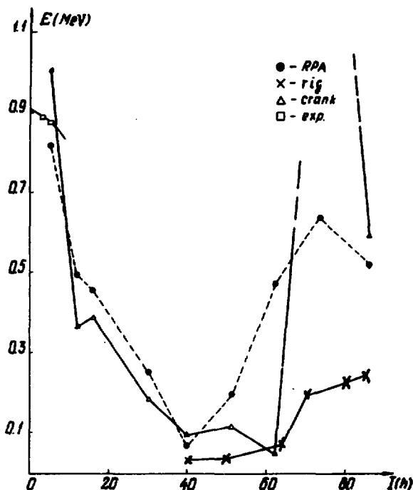
Fig.3. Estimates of the excitation energy of the lowest states with odd I-values in the nucleus ^{168}\text{Yb} . The explanation is given in the text.
