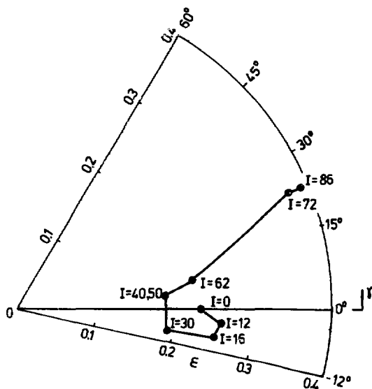
Fig.1. The equilibrium quadrupole deformation in ^{188}\text{Yb} at different spins. The values of spin corresponding to the calculated points are indicated in the plot.
