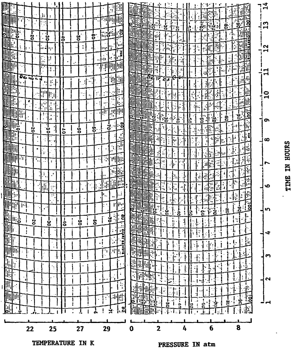
Fig. 24. A picture showing typical records of the bubble chamber operating temperature and pressure under the normal operational condition, recorded on the chart during the seventh operation of the KEK 1 m HBC.
