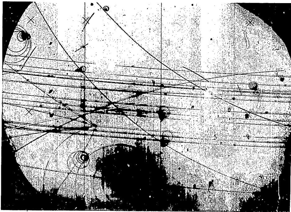
Fig. 25. A typical picture of the 6.0 \text{ GeV}/c \pi^- p interactions.
