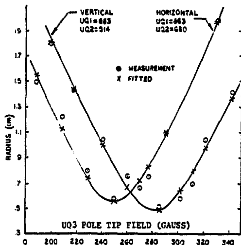
Fig. 5. Beam sizes at U165 as a function of the strength of an upstream quadrupole UQ3.
