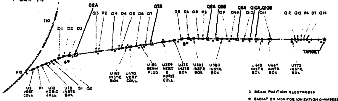
Fig. 3. Plane view of the U-line from the ejector magnet to neutrino production target.
