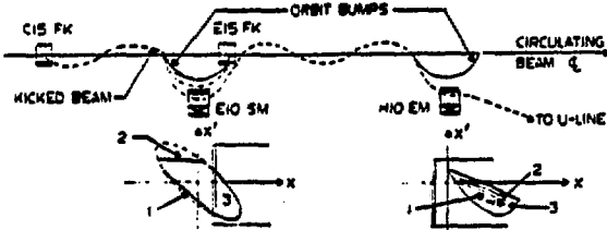
Fig. 1. Schematic layout of the fast extraction configuration and multiturn shaving at E10 SM.
