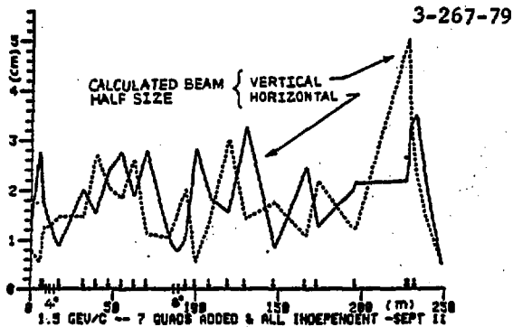
Fig. 6. Calculated beam half size in the U-line.
