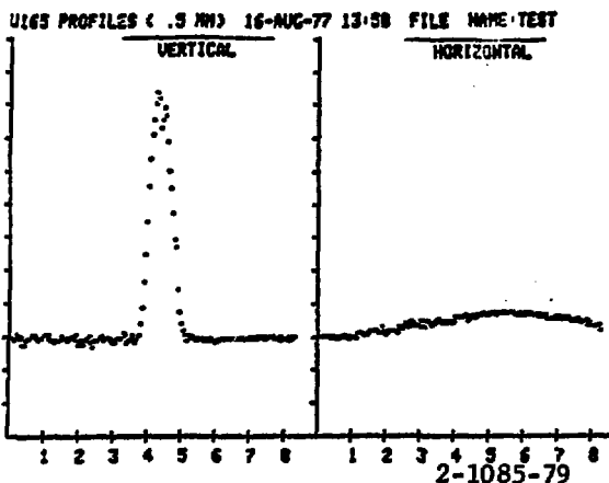
Fig. 4. Beam profile at vertical waist condition.
