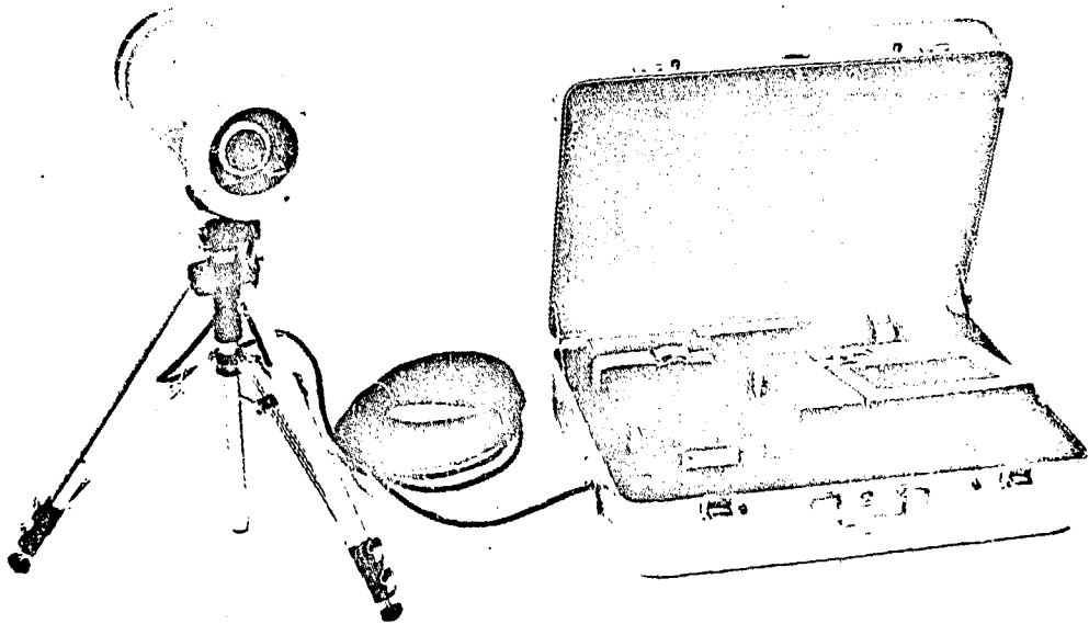
Figure 2. The Portable Battery Power Surveillance and Recording System.
