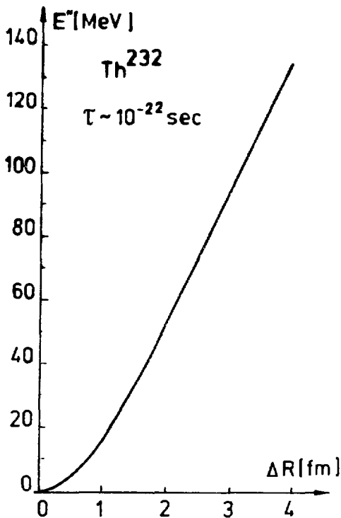
Fig. 2. Dependence of Th^{232} excitation energy E^* ( \tau \approx 10^{-22} sec) in the reaction A_2 + Th ( E_{lab} = 388 MeV) on \Delta R = R_1 + R_2 - R_0 .
