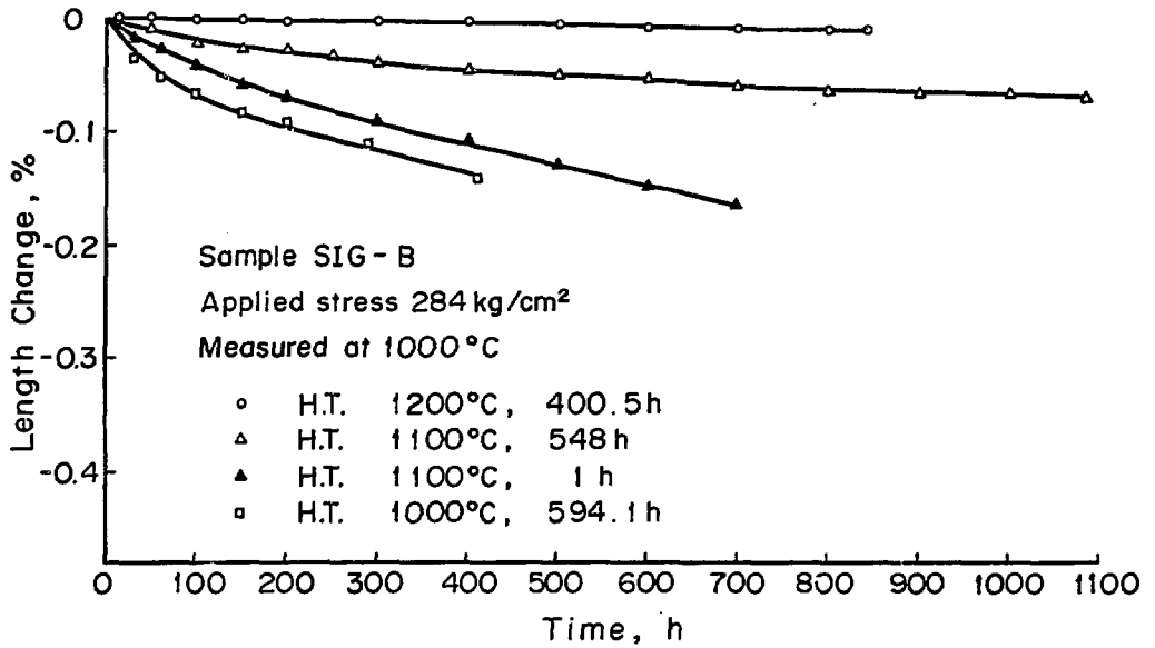
Fig.16 Dimensional changes of the SIG-B carbon heat-treated at 1000°C, 1100°C, 1200°C with time at 1000°C under the compressive stress 284 kg/cm 2 .
