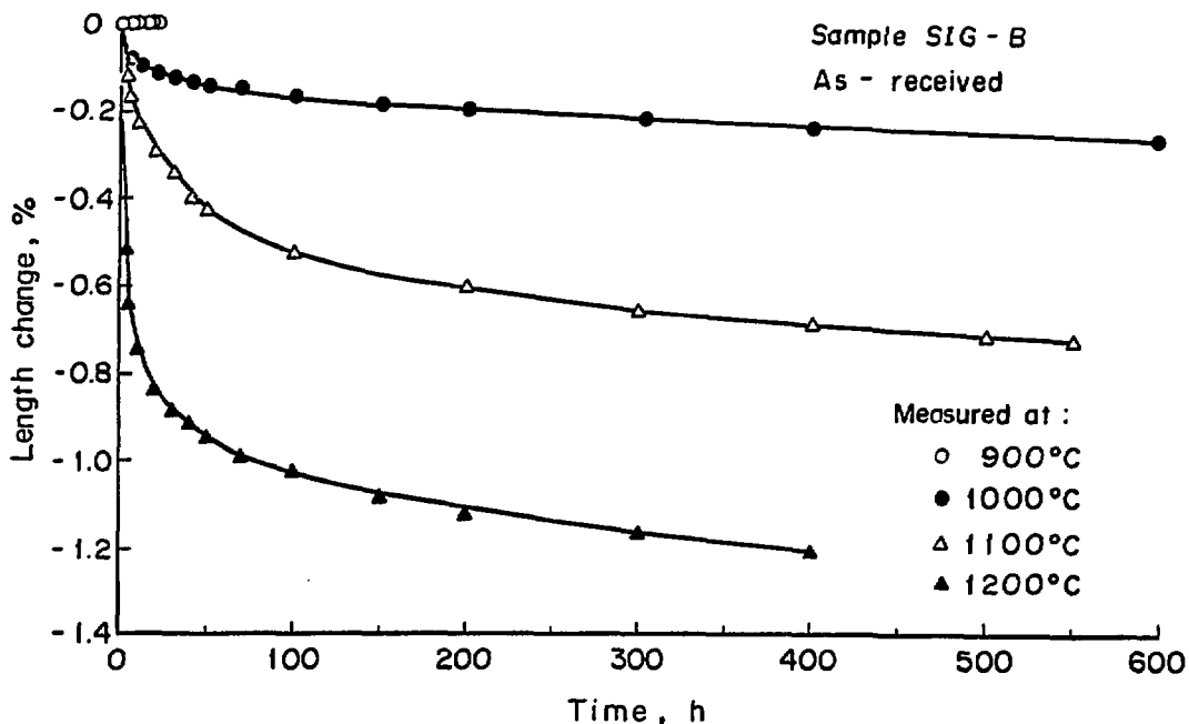
Fig. 6 Dimensional changes of the sample SIG-B with time at 900°C, 1000°C, 1100°C and 1200°C under the compressive stress 3.2 kg/cm².
