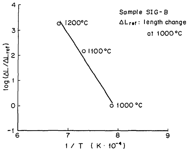
Fig.20 Determination of the activation energy of the sample SIG-B
