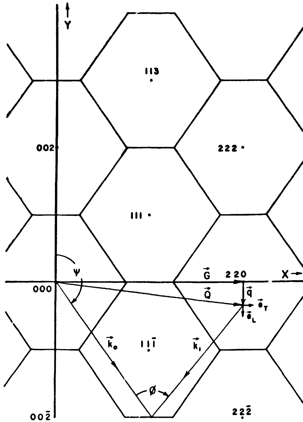
Figure 2 - The (110) plane of copper reciprocal lattice showing a typical inelastic scattering process
