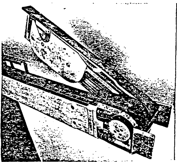
Fig. 2 : The arm raised to a typical operating position with "upper insertion" carrier installed. An empty foil frame can be seen in the position to intercept injected beam.
