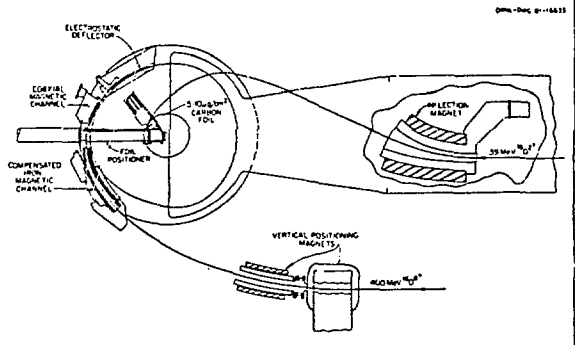
Fig. 1 : Foil positioner shown in position for boosting 16 O 2+ tandem beam to 25 MeV/amu. Pole-tip diameter (dashed circle) is 193 cm.
