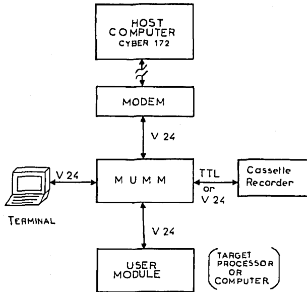
Fig. 1 M.U.M.M. External Interconnections
