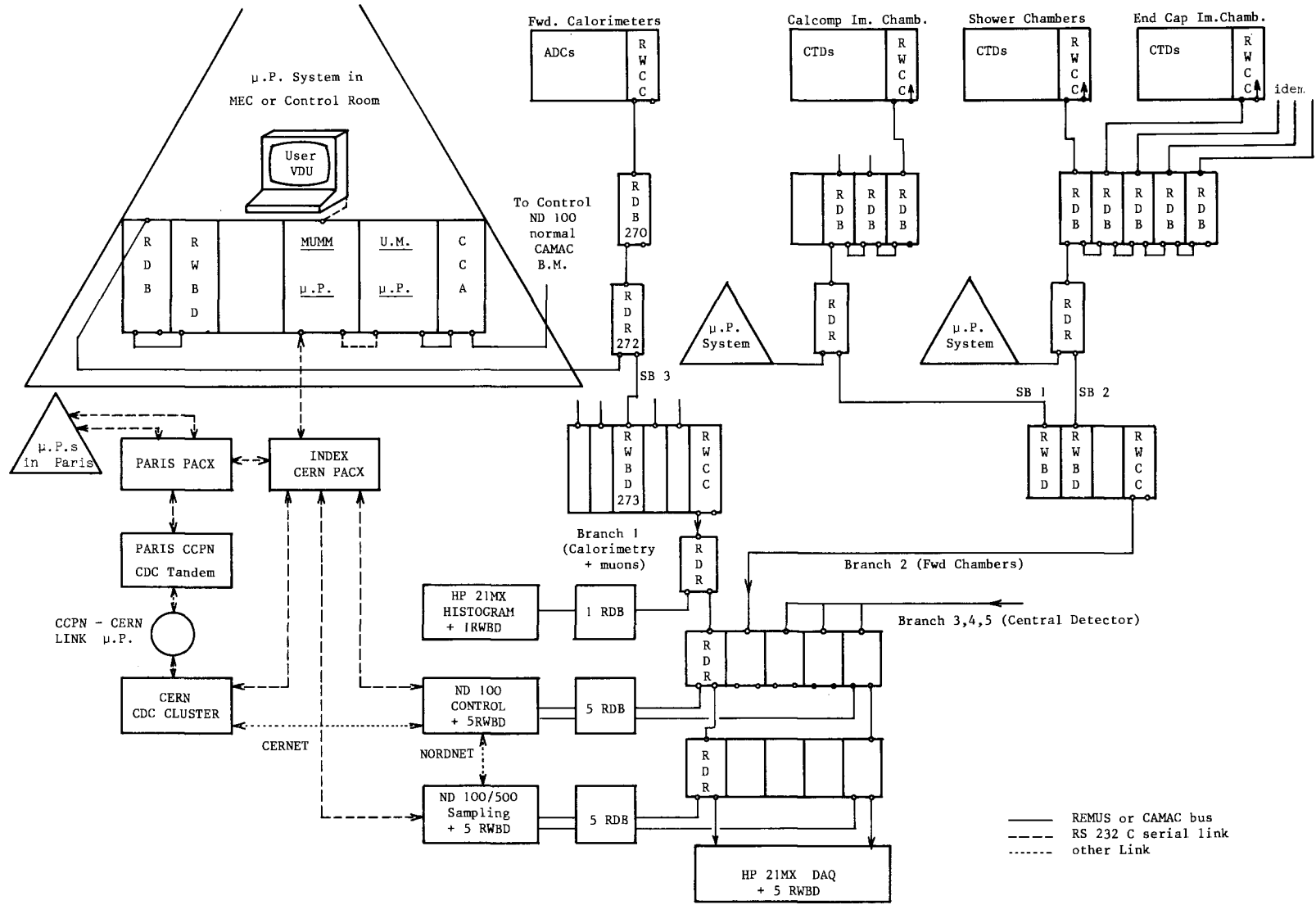
Fig. 3 Control microprocessors implantation in UA1 experiment
