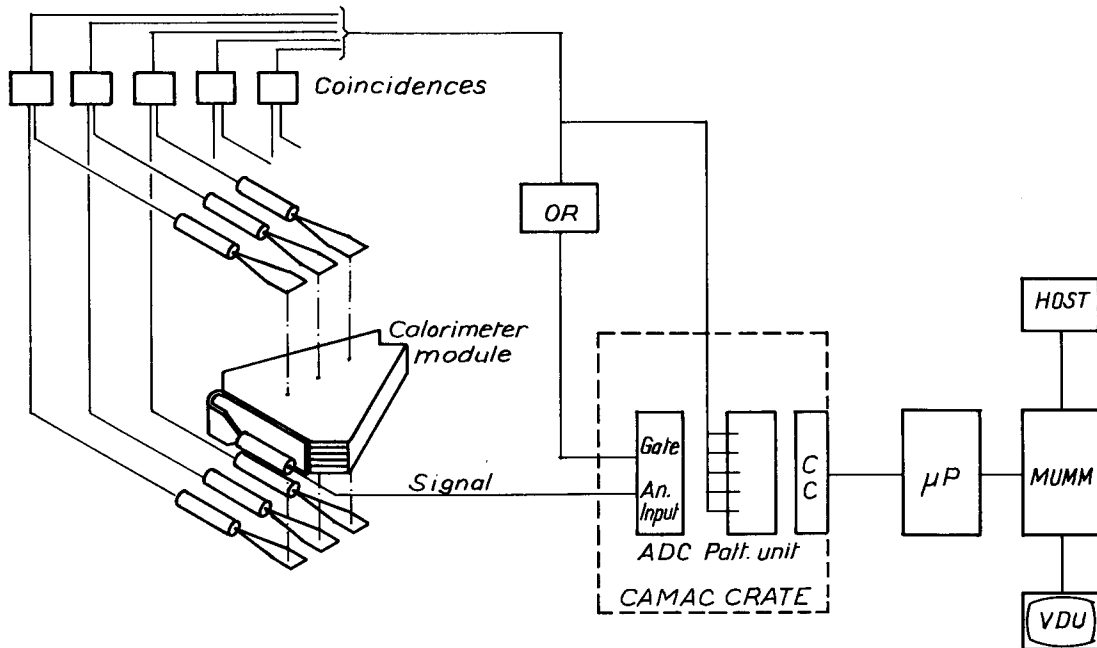
Fig. 1 Typical test-bench application set-up
