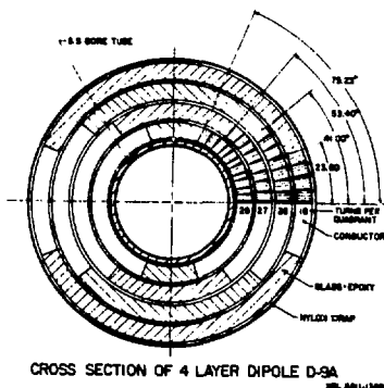
Fig. 1. Cross section of the D-9A Dipole.
