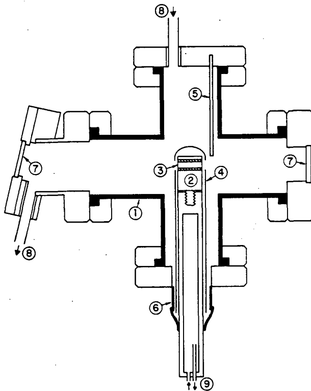
Figure 1. Hollow cathode lamp. 1) Standard 2.75" Diameter Varian Cross. 2) Demountable copper cathode block. 3) Uranium or thorium insert. 4) Quartz shield. 5) Anode rod. 6) Ceramic seal and insulator. 7) Calcium fluoride windows. 8) Argon inlet and outlet. 9) Cooling water inlet and outlet.
