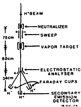
Fig. 2. Schematic diagram of apparatus used by McFarland et al. 3 at LBL (2a) and by Mayo et al. 4 at Wesleyan (2b) to measure charge-state fractions in alkaline-earth vapors.
