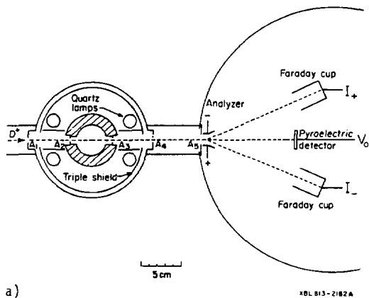
Fig. 2. Schematic diagram of apparatus used by McFarland et al. 3 at LBL (2a) and by Mayo et al. 4 at Wesleyan (2b) to measure charge-state fractions in alkaline-earth vapors.
