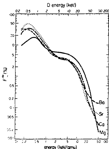
Fig. 8 Summary of equilibrium yields F_{\infty}^{H^-} for H^- formation in alkaline-earth vapors.
