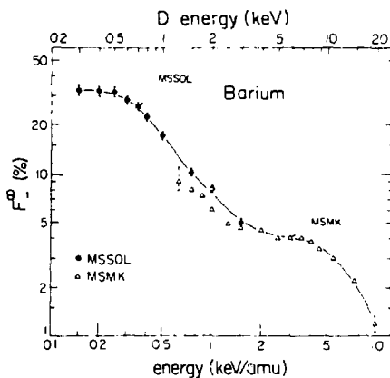
Fig. 7. Equilibrium yield F_{H^-} for H^- formation in barium vapor.
