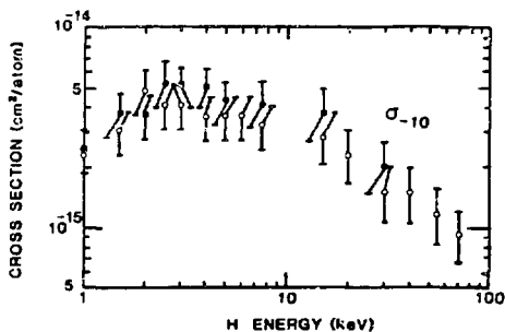
Fig. 11. Electron-detachment cross section \sigma_{-10} for collisions of H^- with calcium ( \bullet ) and strontium ( \circ ) vapors, deduced from measured \sigma_{0-1} and r_{01}^{\infty} .
