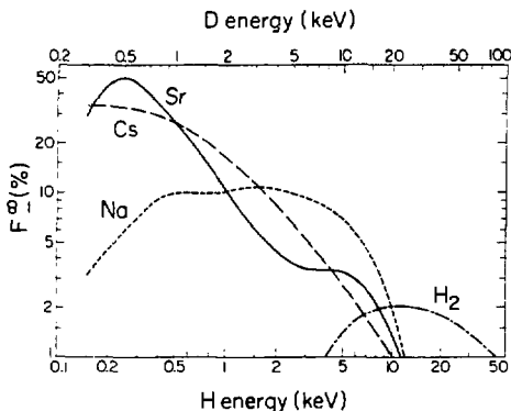
Fig. 1. Summary of equilibrium yields F_{-}^{\infty} for H- formation in typical targets.
