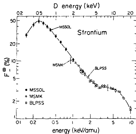
Fig. 6. Equilibrium yield F_{H^-} for H^- formation in strontium vapor.
