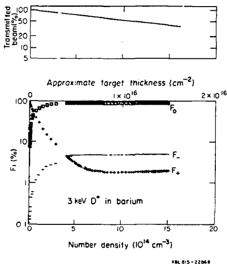
Fig. 3. Charge-state fractions F_i and total transmitted beam as a function of target number and line densities for 1500 eV/amu D^+ incident on barium vapor, from measurements by McFarland et al. 3
