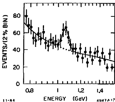
Fig. 12. The \zeta -peak region of the \Upsilon(1S) \rightarrow \gamma + high-multiplicity hadrons, with the fit shown as a solid line. (see text).
