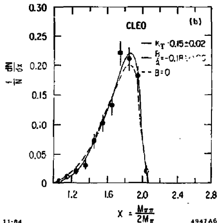
Fig. 6. a) The Argus data for the process \Upsilon' \rightarrow \pi\pi\Upsilon and the MARK II data for the process \psi' \rightarrow \pi\pi J/\psi . The curves show fits to each using the Shifman et al., formulation. b) The CLEO data for the same process with curve parameterized by the Yan, et al., formulation.
