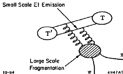
Fig. 5. Elements of the process \Upsilon' \rightarrow \pi\pi\Upsilon .
