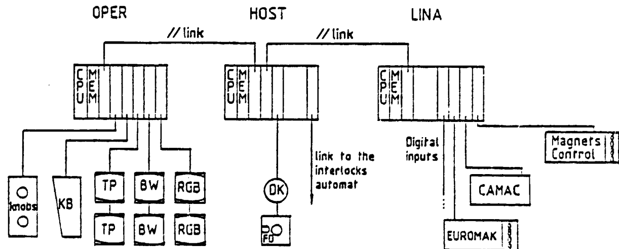
Hardware Configuration
