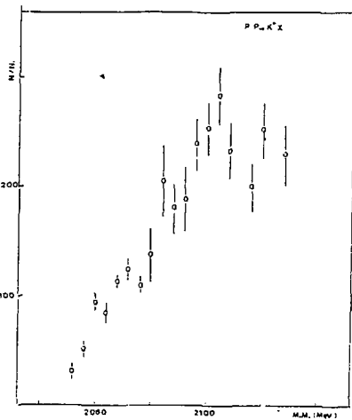
Fig. 6 : Preliminary pp \rightarrow K^*X missing mass spectrum obtained at \theta = 8^\circ and T_p = 2.5 GeV.
