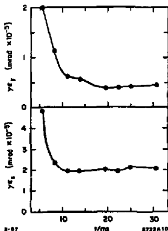
Fig. 5. The emittance of the beam extracted from the electron storage ring as a function of storage time. The vertical emittance \gamma_{e_y} is smaller than the horizontal emittance because the ring is operated without coupling.
