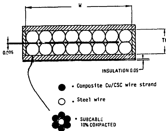
Figure 2 Wire based cable detail.
