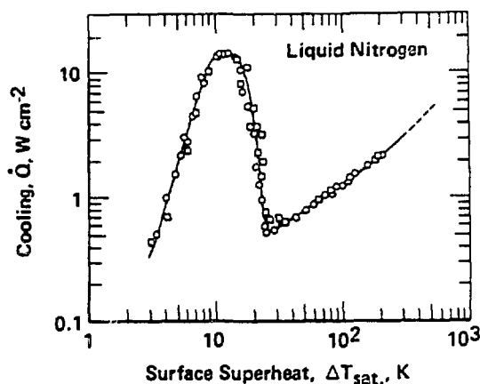
Figure 1. Heat transfer to liquid nitrogen.
