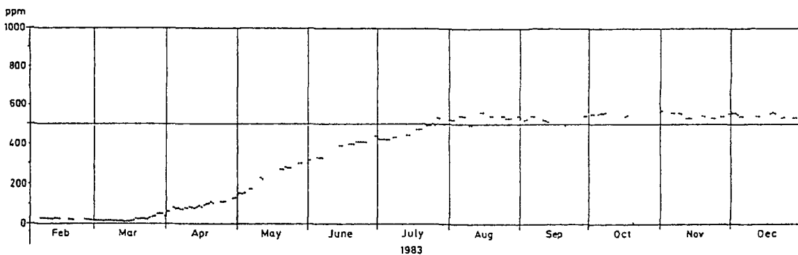
Figure 11 Ruth - ISL Chloride (Cl - ) in Recovery Stream, Leaching Phase
