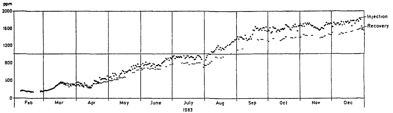
Figure 10 Ruth - ISL Bicarbonate (HCO 3 - ) in Recovery and in Injection Stream, Leaching Phase
