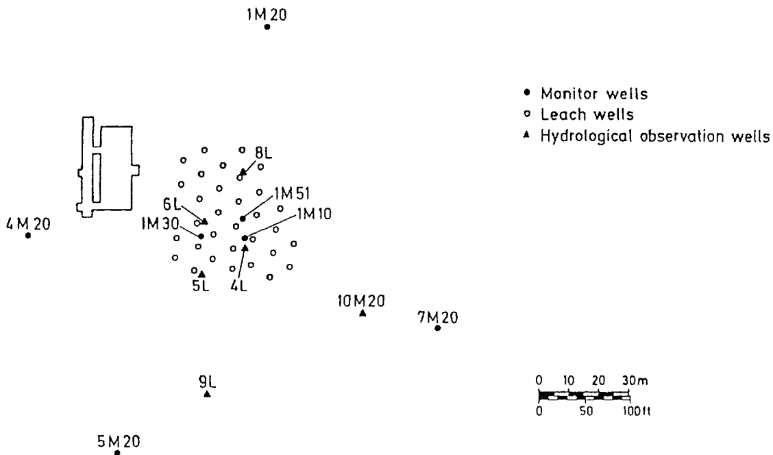
Figure 5. Ruth-ISL Well Locations
