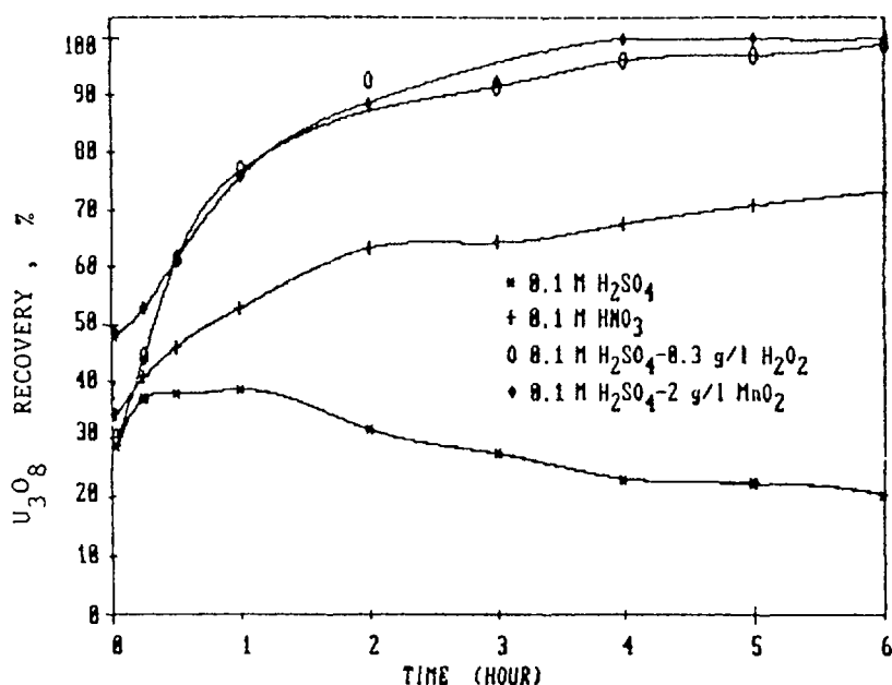
Figure 3- Comparison of \text{U}_3\text{O}_8 Recovery For Several Acid Leach Tests
