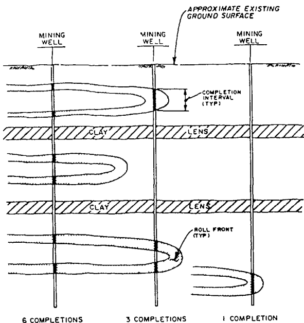
FIGURE 3 SCHEMATIC REPRESENTATION OF MULTI-ZONE MINING
