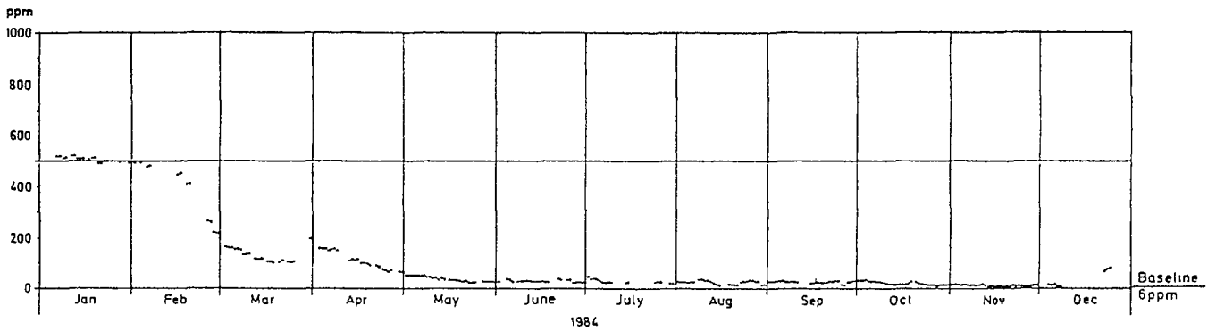
Figure 17 Ruth - ISL Chloride (Cl - ) in Recovery Stream, Restoration Phase
