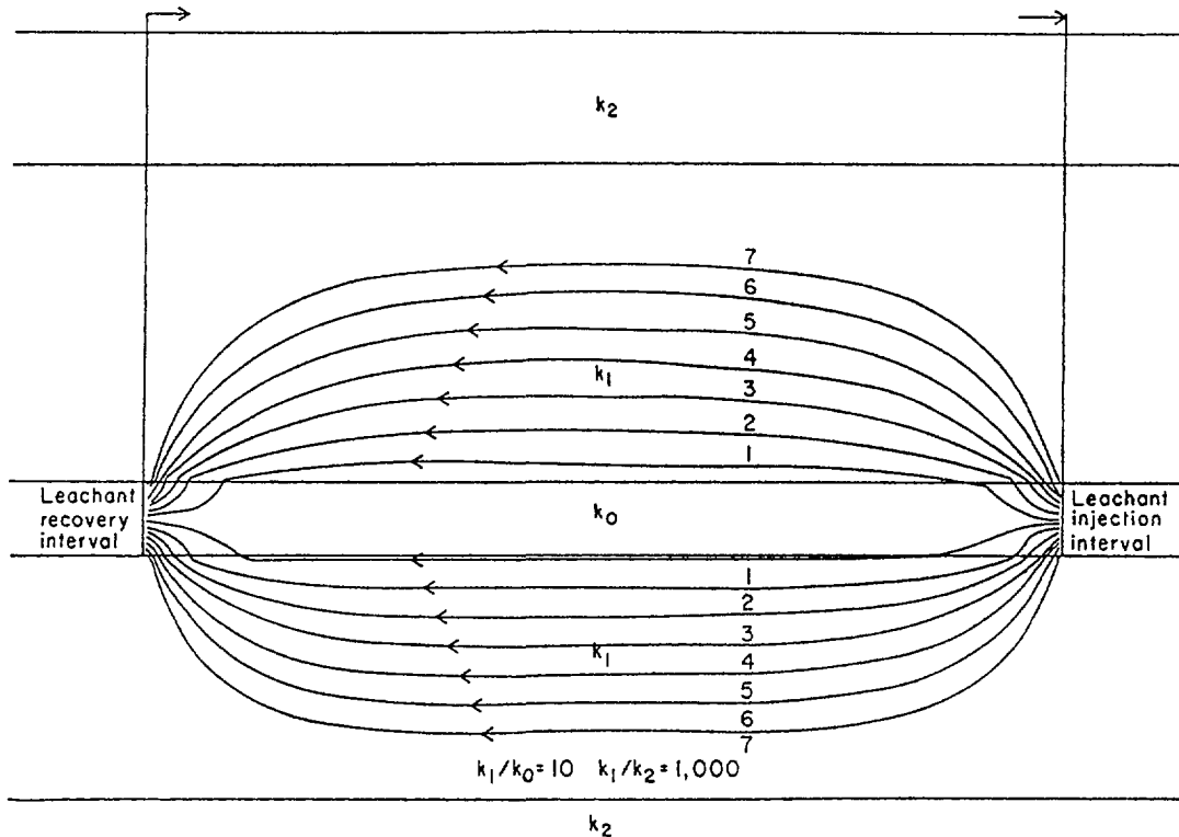
FIGURE 3. - Streamline pattern in a heterogeneous cross section (26).
