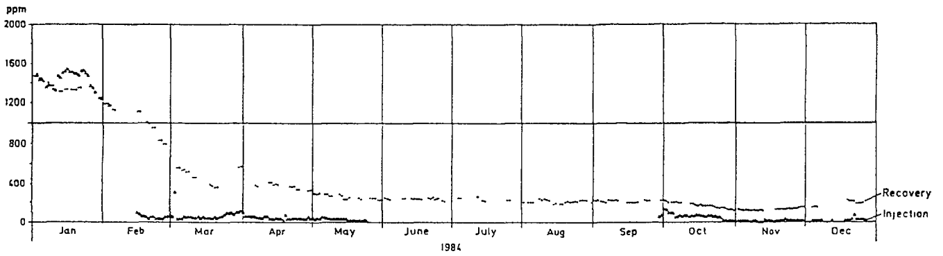
Figure 16 Ruth - ISL Bicarbonate (HCO 3 - ) in Recovery and in Injection Stream, Restoration Phase
