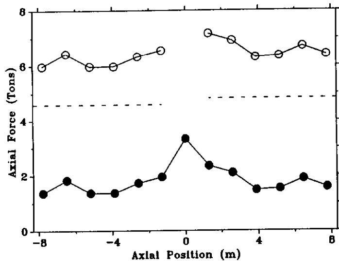
Fig. 2. Axial Lorentz force carried by the cold mass skin (closed circles) and by the coil (dashed lines) in DD0015. Open circles show the sum. Plot boundaries represent the magnet ends.
