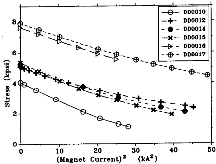
Fig. 1. Inner coil stress versus magnet current squared. Data displayed are an average of four measurements on the left and right sides of the upper and lower coils at a location where the stress is expected to be smallest.
