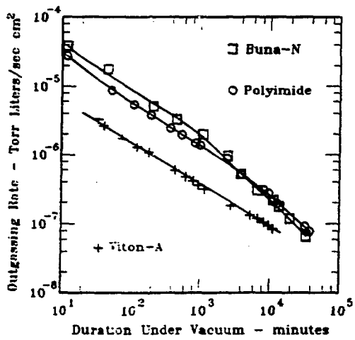
Fig. 6. Outgassing Rate of Three Popular Elastomers as a Function of Time in Vacuum.
