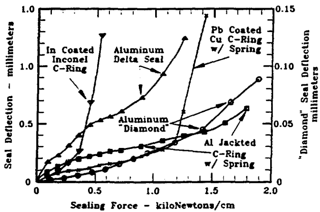
Fig. 3. Seal Deflection as a Function of Sealing Force. (Right Scale for "Diamonds"; Left Scale all Other Seals)
