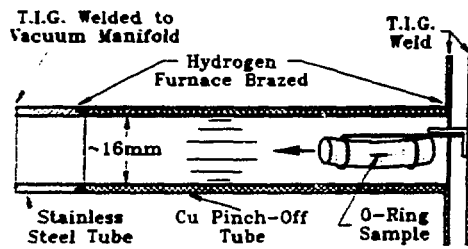
Fig. 4. Copper Pinch-off Assembly Used to House O-Ring Test Sample for Extended Vacuum Exposure.
