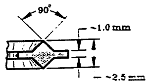
Fig. 2. Minor Dimensions of the 1100 Aluminum "Diamond Seal" used in the Seal Test Program.
