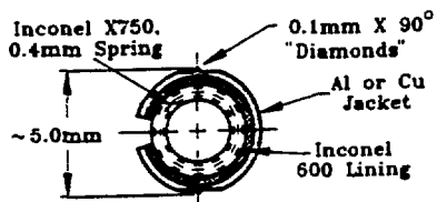
Fig. 1. Approximate Minor Dimensions of Helicoflex Delta ® Seal used in the AGS.
