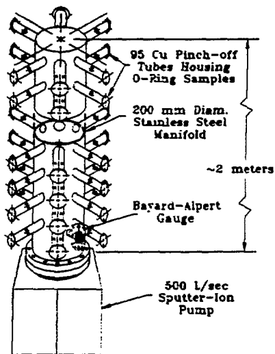
Fig. 5. Apparatus Used to Evaluate the Long Term Effects of Elastomer Exposure to Vacuum.
