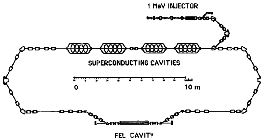
Fig. 1 - View of LISA layout.
