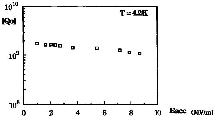
Fig. 3 - Quality factor vs. accelerating field for single cell 500 MHz cavity.
