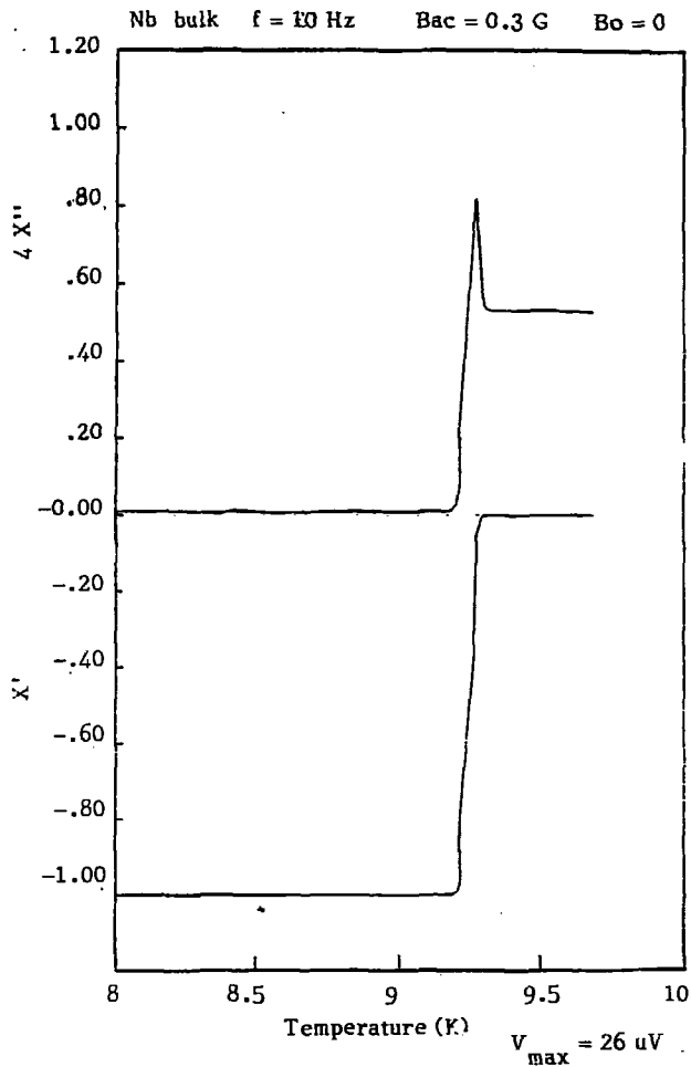
Fig. 6 - Real and imaginary parts of susceptibility vs. temperature.
