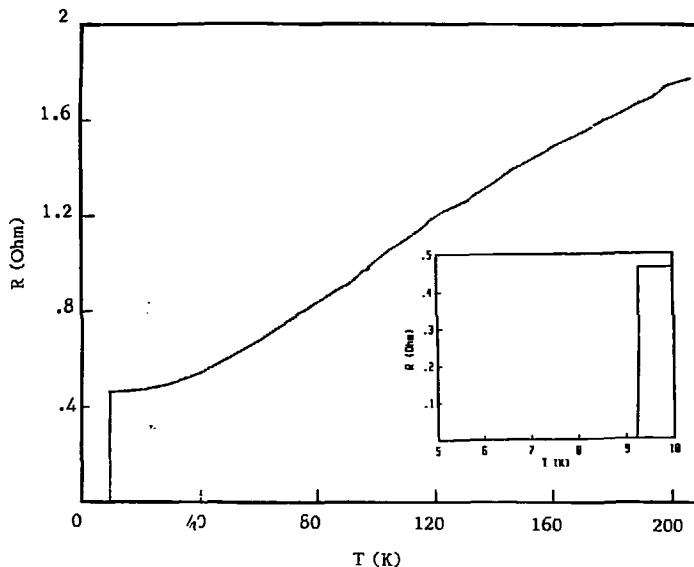
Fig. 4 - Resistance vs. temperature for Nb thin film.
