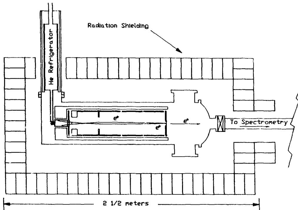
Figure 1. Schematic diagram of krypton irradiation loop, slow positron source cup, Soa lens, and brightness enhancement film. Details of source cup, Soa lens, and brightness enhancement film shown in upper left diagram.
