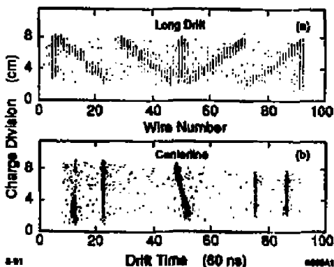
Fig. 2: Representative results from UV fibers on TPCs: (upper) in a plane parallel to the detector wire plane; and (lower) in a plane down the centerline of the TPC.
