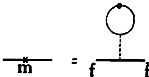
Fig. 1 - Fermion mass gap equation in terms of the scalar boson tadpole graph
