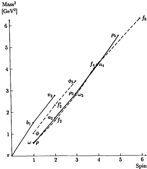
Figure 2: Lowest-lying experimental Regge trajectories for non-strange mesons [16]
