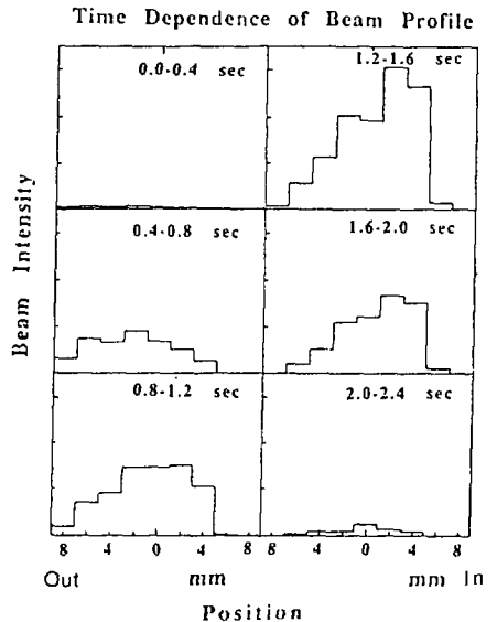
Fig. 3 Time dependence of the horizontal profile of the extracted beam.
