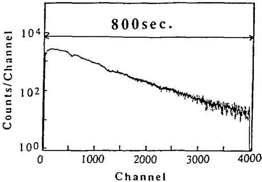
Fig. 5 Spill of the beam extracted by the utilizing the emittance growth due to the multiple scattering with residual gases in the ring.
