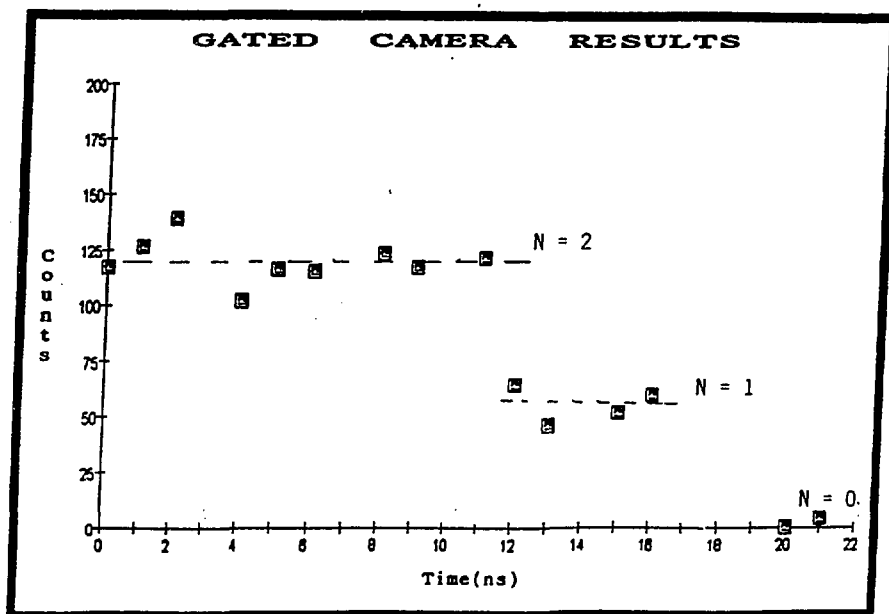
Fig. 3. Gated camera results from SSRL show observation of single electron bunch ( N=1 ) is possible with visible synchrotron radiation.
