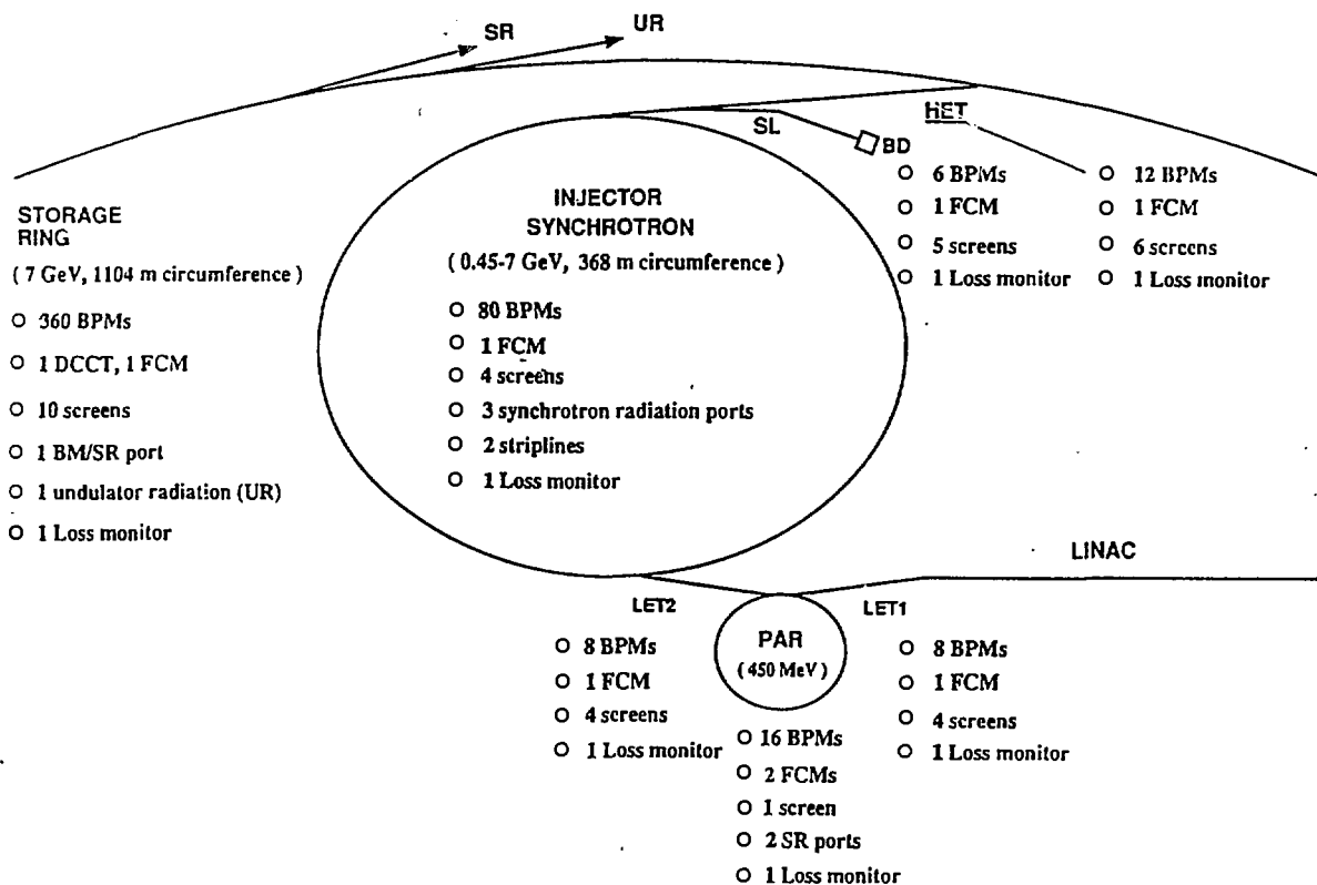
Fig. 1. A schematic of the APS subsystems showing the diagnostics for those other than the two linacs.
