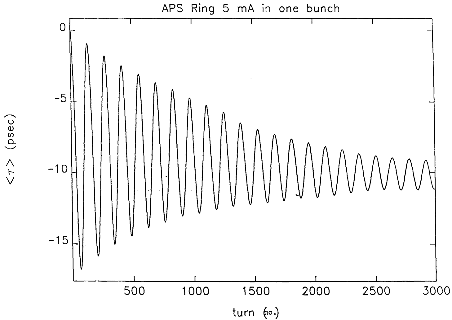
Fig. 5. Simulation of the variation of bunch phase during damping in the storage ring.
