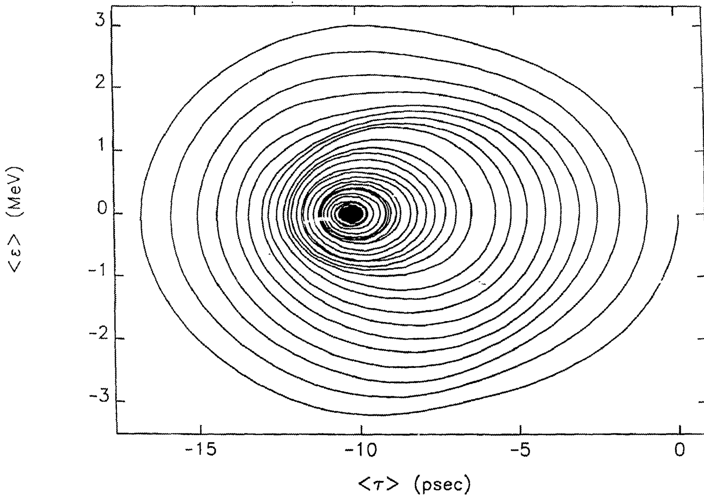
Fig. 6. Simulation of the longitudinal phase space (average energy and average phase) damping dynamics in the storage ring.
