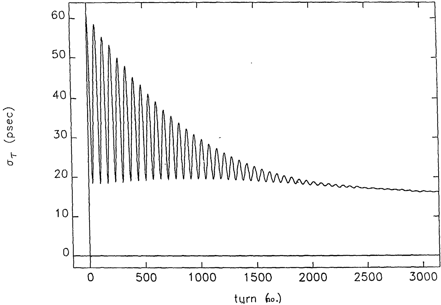
Fig. 4. Simulation of the damping of the positron bunch's temporal length versus turn number in the storage ring.
