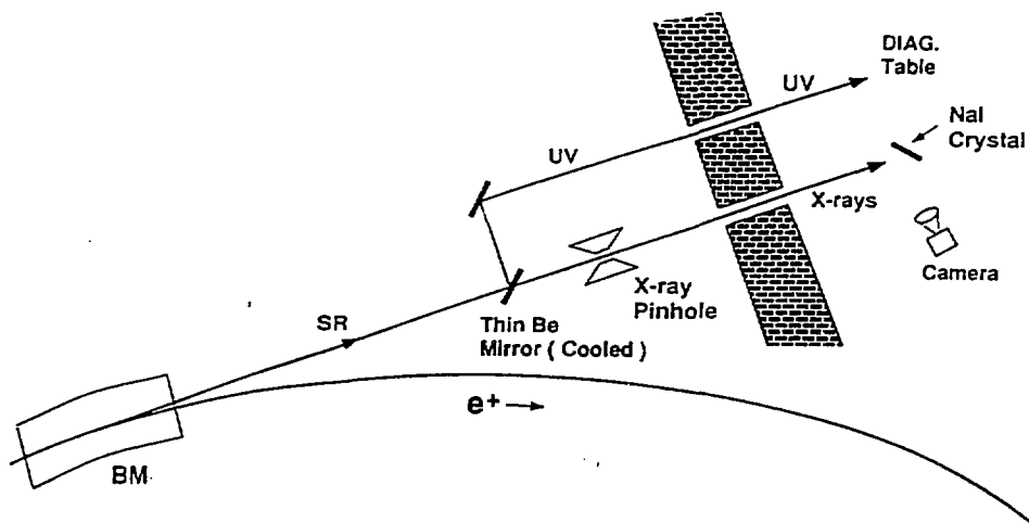
Fig. 2. A schematic of the positron beam imaging via bending magnet synchrotron radiation (UV and X-ray components).
