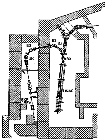
Figure 1: CAD lay-out of the BTF-line
