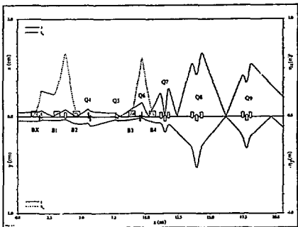
Figure 2: Optimized lattice for the plasma lens experiment.
