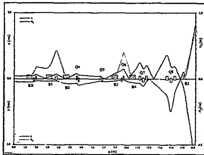
Figure 3: Optimized lattice for the X-ray source experiment.
