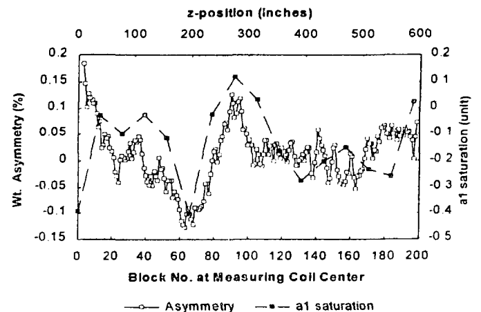
Fig.3 Variation of Top-bottom weight asymmetry and \delta a_1 along the length of the magnet DCA213
