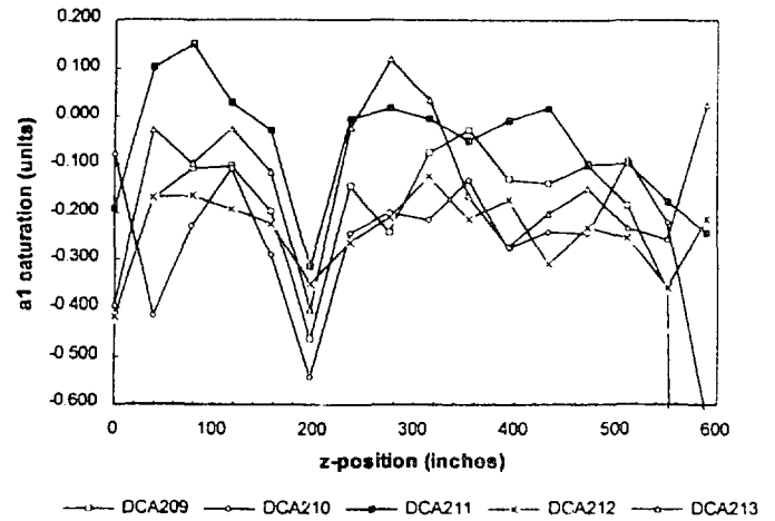
Fig.2 a_1 saturation ( \delta a_1 ) in DCA209-DCA213 Magnets
