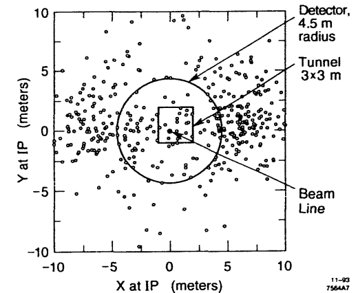
Figure 7. Spatial distribution of muons which reach the IP from six sources in the collimation section.
