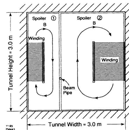
Figure 3. Two side-by-side magnetized iron spoilers filling a 3 x 3 meter beam tunnel.
