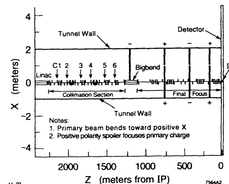
Figure 2. Plan view of the NLC beam line in the tunnel with magnetized iron spoilers.
