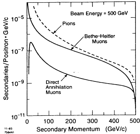
Figure 1. Secondary muon and pion yields from 500 GeV electrons and positrons incident on a 20 r tungsten target.
