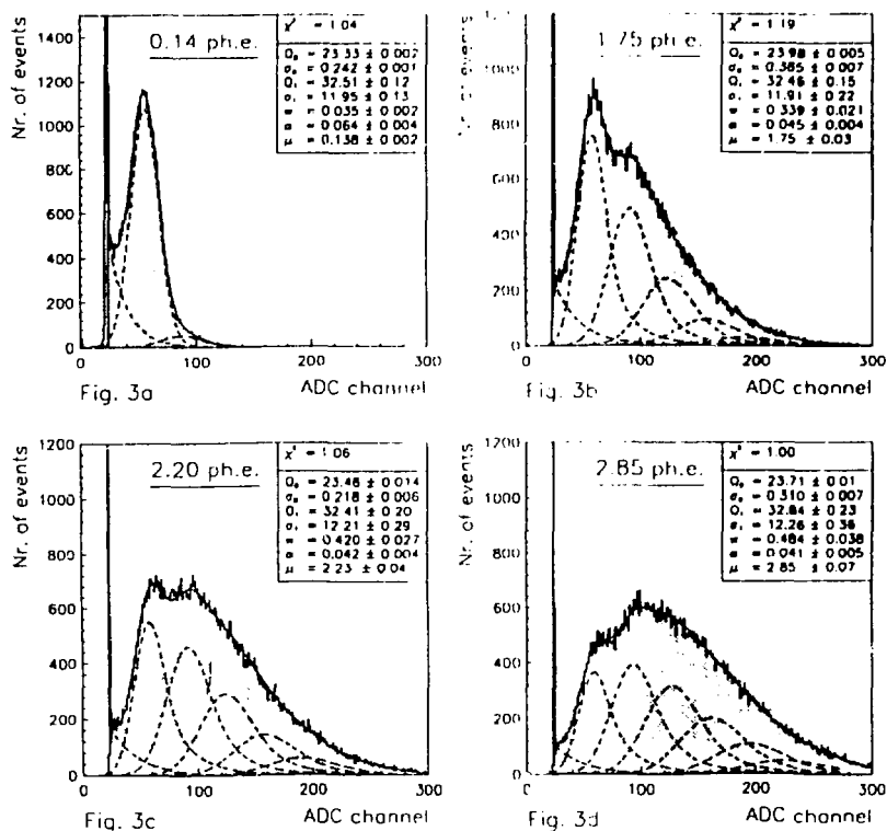
Fig. 3 LED spectra taken with a EMI-9814B photomultiplier constant voltage for different intensity of light source (0.1 - 6.7 photoelectrons).
