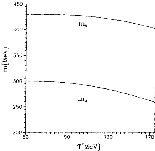
Figure 4: The T -dependence of m_u and m_s with gluon condensate
