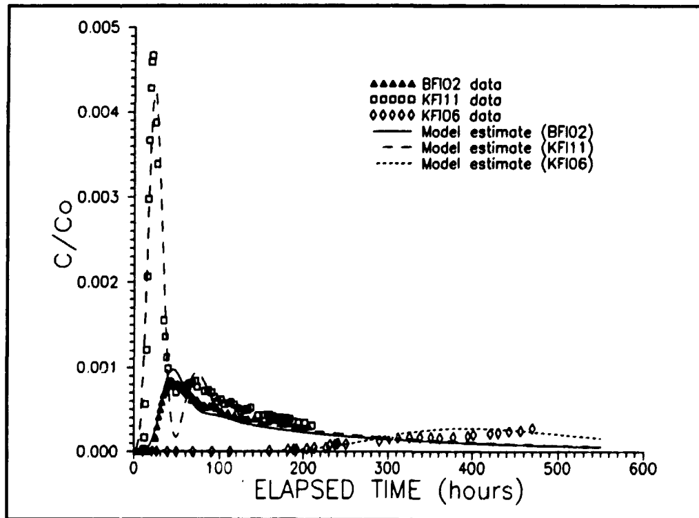
Figure 3-3. Results of estimation using data from all boreholes simultaneously, assuming anisotropic hydraulic conditions and aerially distributed vertical leakage. /Andersson et al., 1993/.
