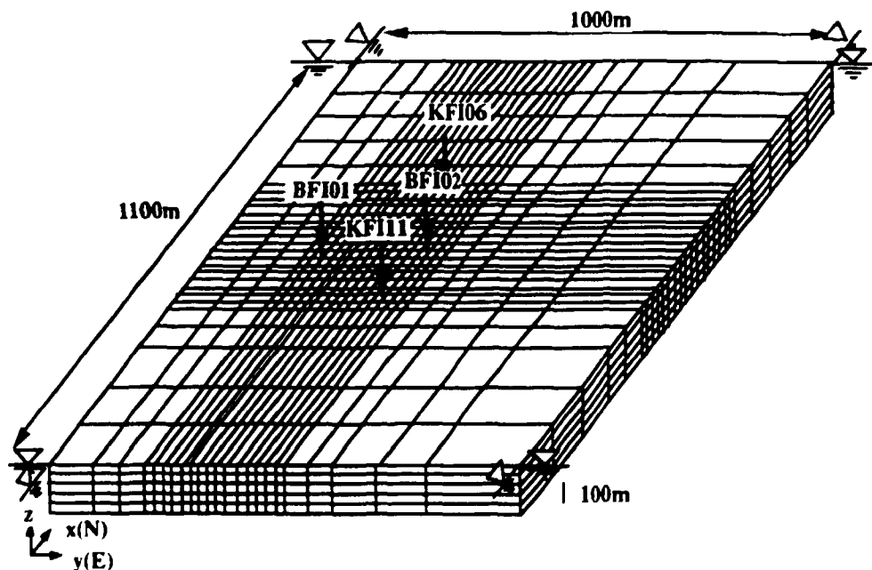
Figure 3-22. Schematic view of the finite element mesh and boundary conditions applied in the numerical analysis
