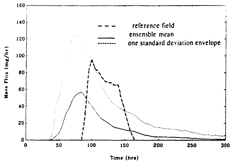
Figure 3-25. Ensemble mean breakthrough curve at BFI02, Case 2 - particles released at KFI11 (porosity n=0.025 )
