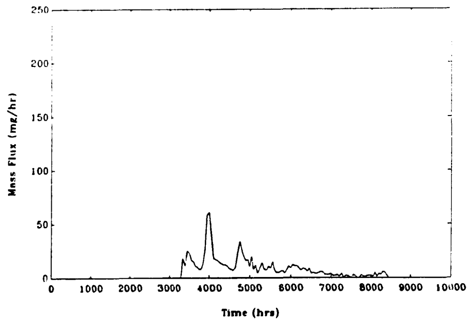
Figure 3-26 Far-field breakthrough curve for realization #22.
