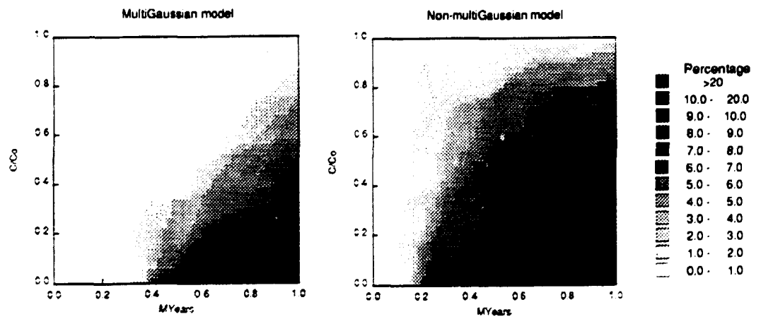
Figure 3-34. Bivariate cumulative probability distribution functions for mass concentration and arrival time (probability of concentration higher than a given value arriving at the surface before a given time).
