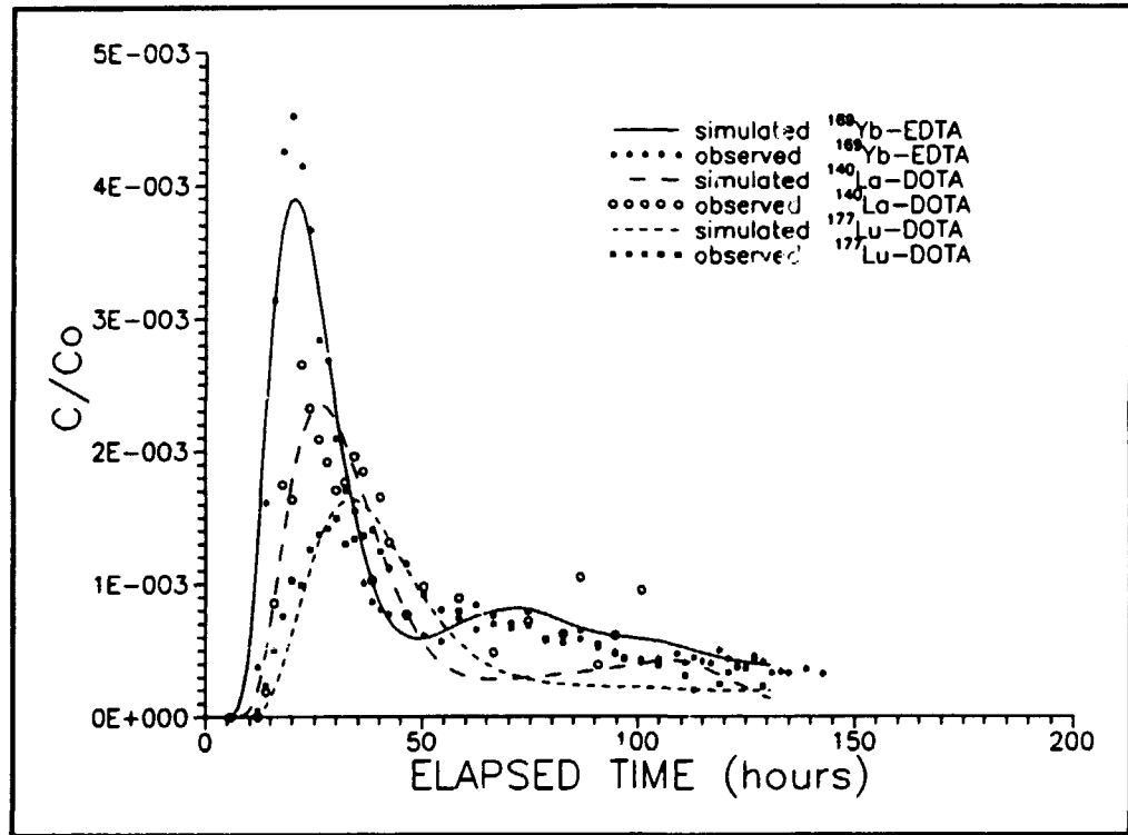
Figure 3-2. Simultaneous model simulation of breakthrough in borehole KFI11 for ^{169}\text{Yb-EDTA} , ^{140}\text{La-DOTA} , and ^{177}\text{Lu-DOTA} /Andersson et al., 1993/.
