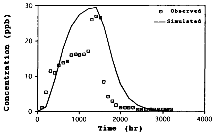
Figure 3-17. Comparison between simulation with the single porosity model and observed breakthrough data for In-EDTA (BFI01:U) /Ng & Kota, 1993/.
