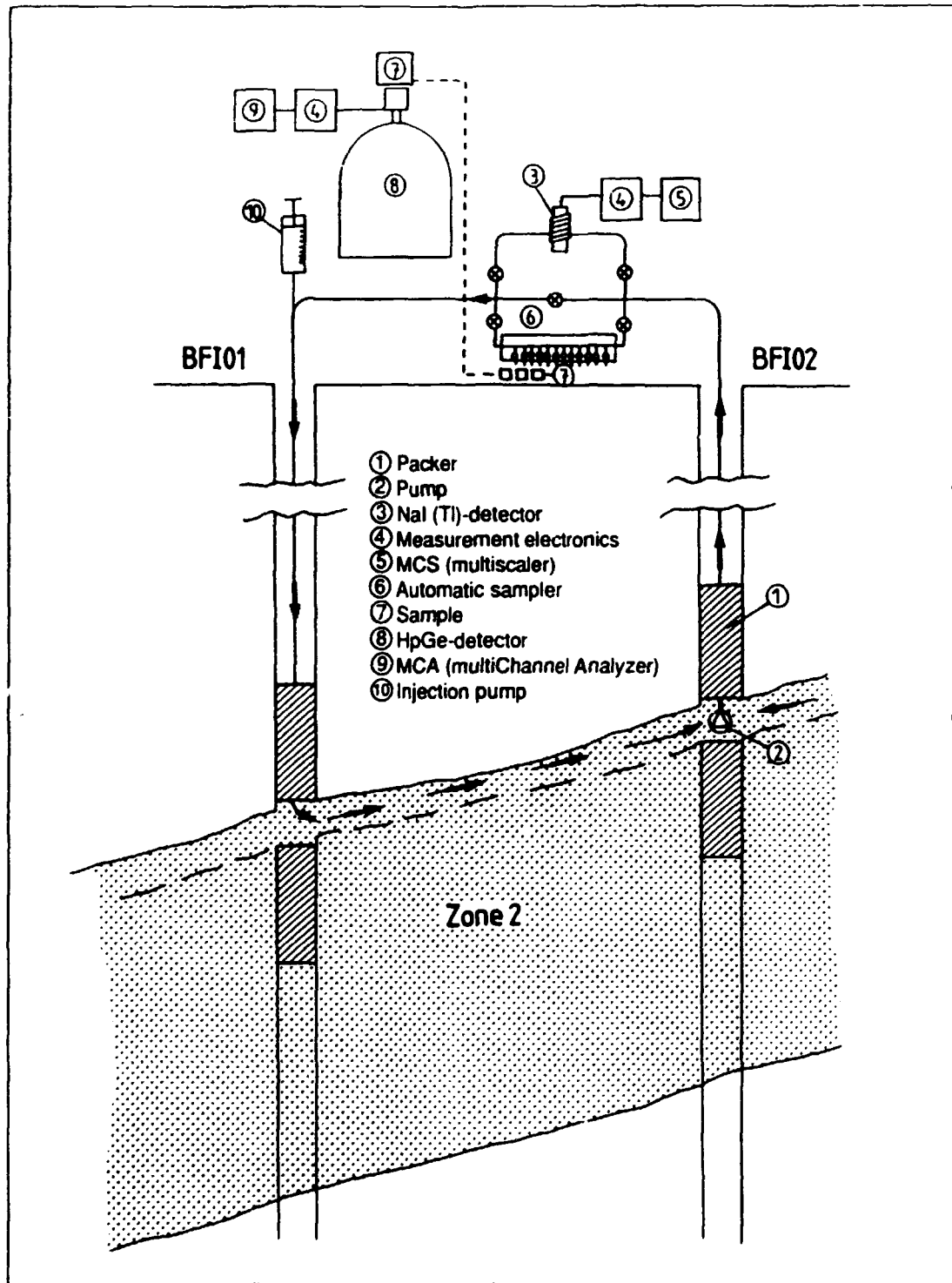
Figure 2-4. Experimental design of the dipole experiment. From Andersson et al. (1993).
