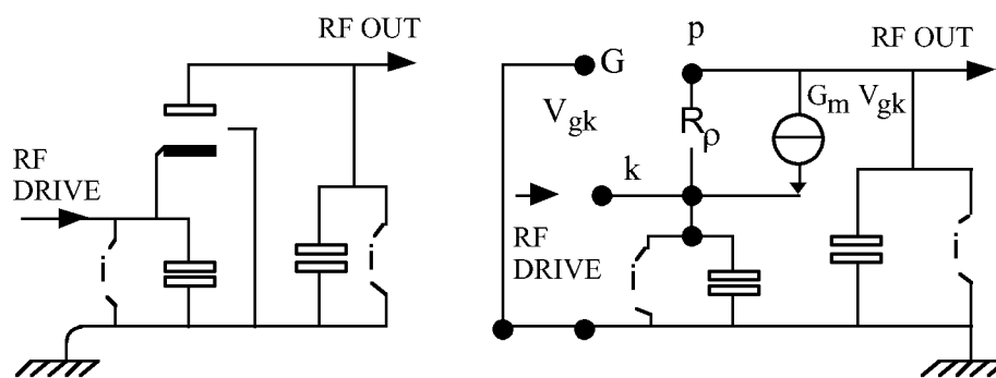
Fig. 23 Grounded-grid configuration
