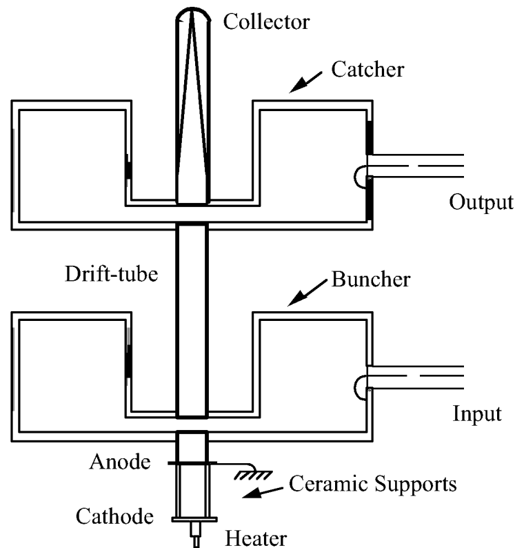
Fig. 25 Schematic of a klystron amplifier
