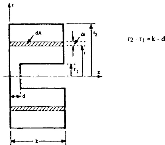
Fig. 9 Cross section of 'LC' cavity with the gap on one side
