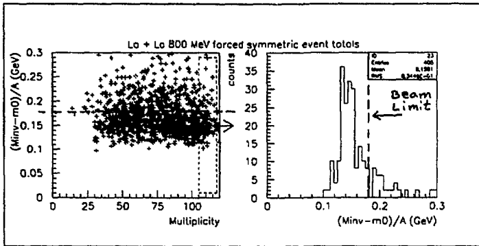
Fig. 4: The quantity (M_{inv} - M_0)/A_{measured} as a function of the event multiplicity. Only the particles in the forward half of the CM frame have been used and reflected into the back half to create a full event. The right hand frame shows a histogram of the highest multiplicity portion of the scatter plot projected onto the (M_{inv} - M_0)/A_{measured} axis.
