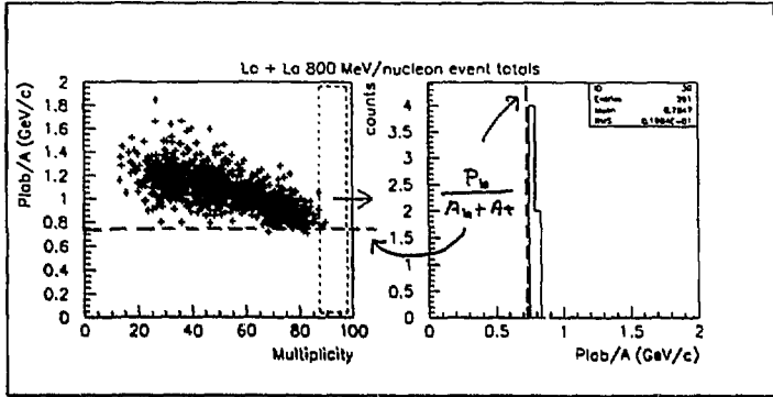
Fig. 5: The measured quantity, p_{lab}/A_{measured} is shown as a function of multiplicity. The limiting value, p_{lab}/(A_{beam} + A_{target}) , that would be seen if all the particles were detected is shown for comparison.
