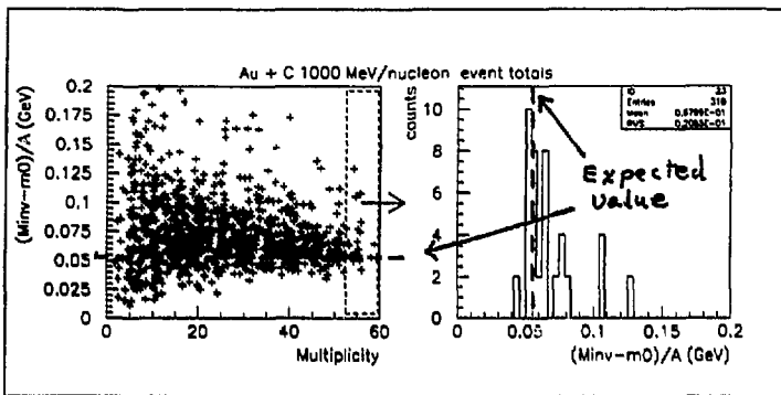
Fig. 6: The quantity, (M_{inv} - M_0)/A_{measured} , is shown as a function of multiplicity for the 1000 MeV* A Au + C system. The expected value, if all the energy is accounted for, is shown for comparison.
