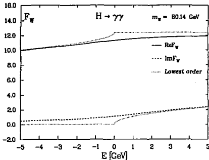
Fig. 2. W -loop form factor F_W^H of the scalar Higgs decays h, H \rightarrow \gamma\gamma plotted versus the distance E = m_H - 2m_W to the W^+W^- -threshold. The results including the decay width \Gamma_W are compared to the lowest order perturbative ones.
