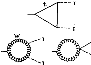
Fig. 1. Generic Feynman diagrams of the H\gamma\gamma and A\gamma\gamma couplings in lowest order: (a) top-loop contributing to the scalar H\gamma\gamma and the pseudoscalar A\gamma\gamma coupling, (b) W -loop contributing to the scalar H\gamma\gamma coupling.
