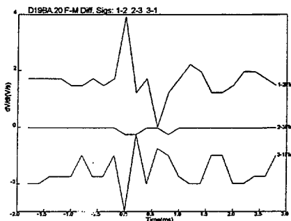
Fig. 4. Fast-Motion: Axial localization is visible from the difference signals of coils #1 (food-end), #2 (middle), and #3 (return-end). Signal 2-3 is quiet, while 1-2 is a rough inverse of 3-1. Hence, the signal-source is within region #1.
