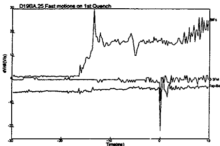
Fig. 6. 1st quench (#24): The largest fast-motion transient produced the stop-trigger ( t = 0 ) but occurred 17 ms after quench-initiation (BIFs @ t = -17 ms). A smaller one was coincident with quench onset.
