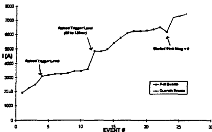
Fig. 2. Training curve: Magnet Current (A) vs. Training Event #. Considerable "training" occurred before the first quench (#24). Restarting the ramp from I=0 (#23) showed only a small fall-back.
