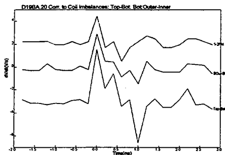
Fig. 5. Fast Motion: The antenna-imbalance (1-2) onset was coincident with one or more magnet-coil-imbalance (both imbalances in this example, same event as Fig. 5).
