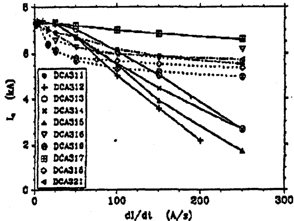
Figure 2. Ramp rate ( di/dt ) dependance of quench current.
