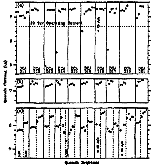
Figure 1. Spontaneous quench performance on the first (a) and second (b) cooldown at 4.35 K, and on the second cooldown at 3.85 K and 3.50 K (c). Closed (open) circles indicate quenches originating in the inner (outer coil).
