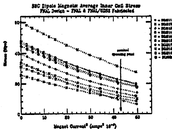
Figure 3. Azimuthal coil stress as a function of I^2 for all tested magnets. Data taken at 4.35 K during the first thermal cycle.
