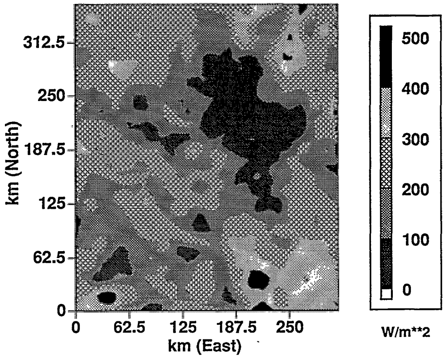
Figure 1. Heat fluxes derived from the SiB2 model for July 28, 1994.
