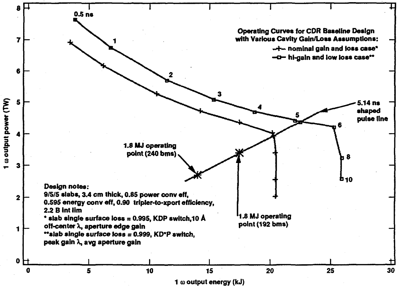
Figure 5. 1.053 μm (1ω) performance curve for the optimized 9-5-5 amplifier design.
