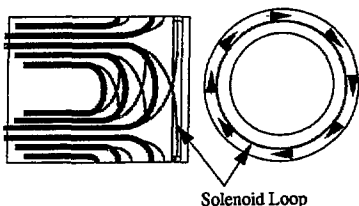
Fig. 5 Unwanted Solenoid Loop
