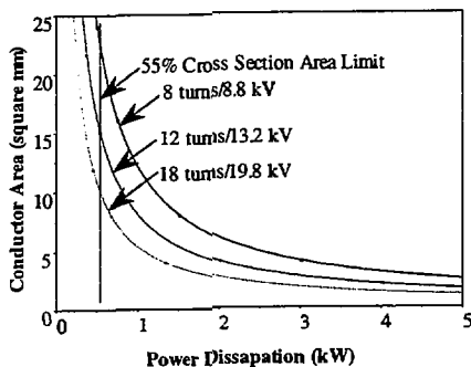
Fig. 3 Conductor size versus energy loss
