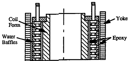
Fig. 2. The Magnetic Quadrupole Cooling Jacket
